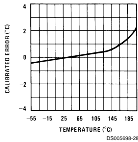
Calibrated Error
