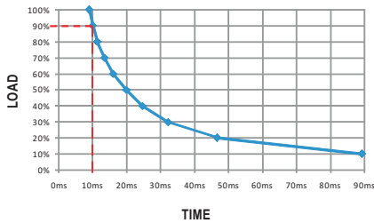
RSD-300B-48
